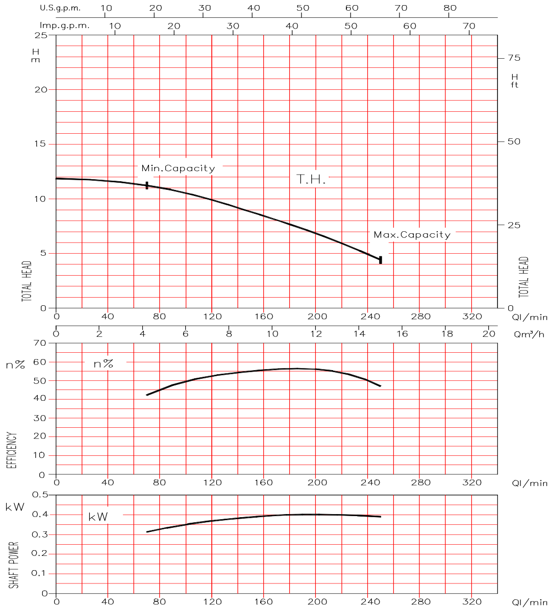
LPS 40/40 (0.4 kW) - LPS 40/40M (0.4 kW) - Impeller diameter = 103 mm
