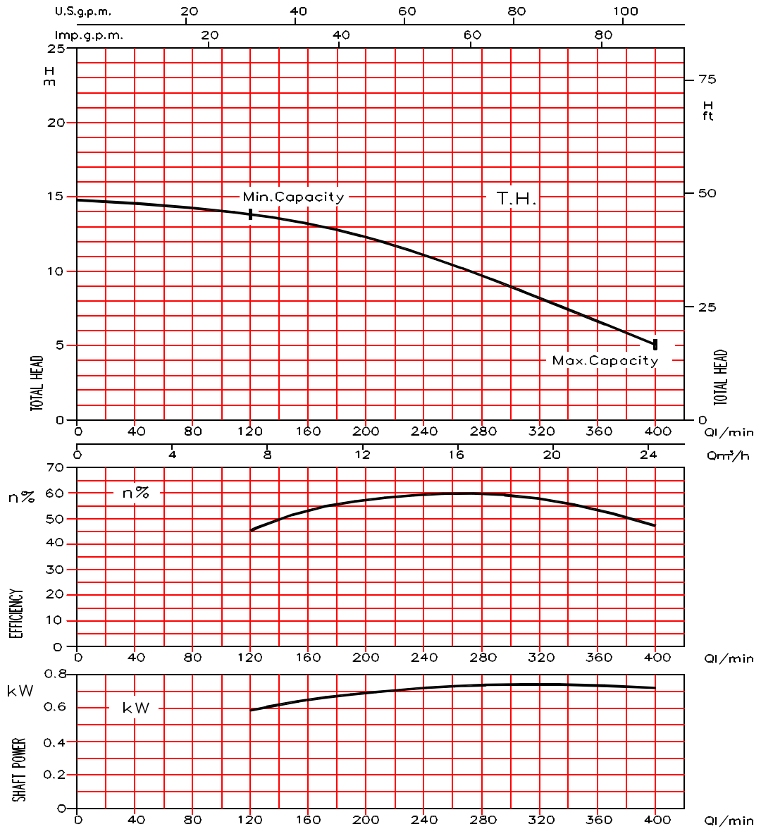
LPS 50/75 (0.75 kW) - LPS 50/75M (0.75 kW) - Impeller diameter = 114 mm
