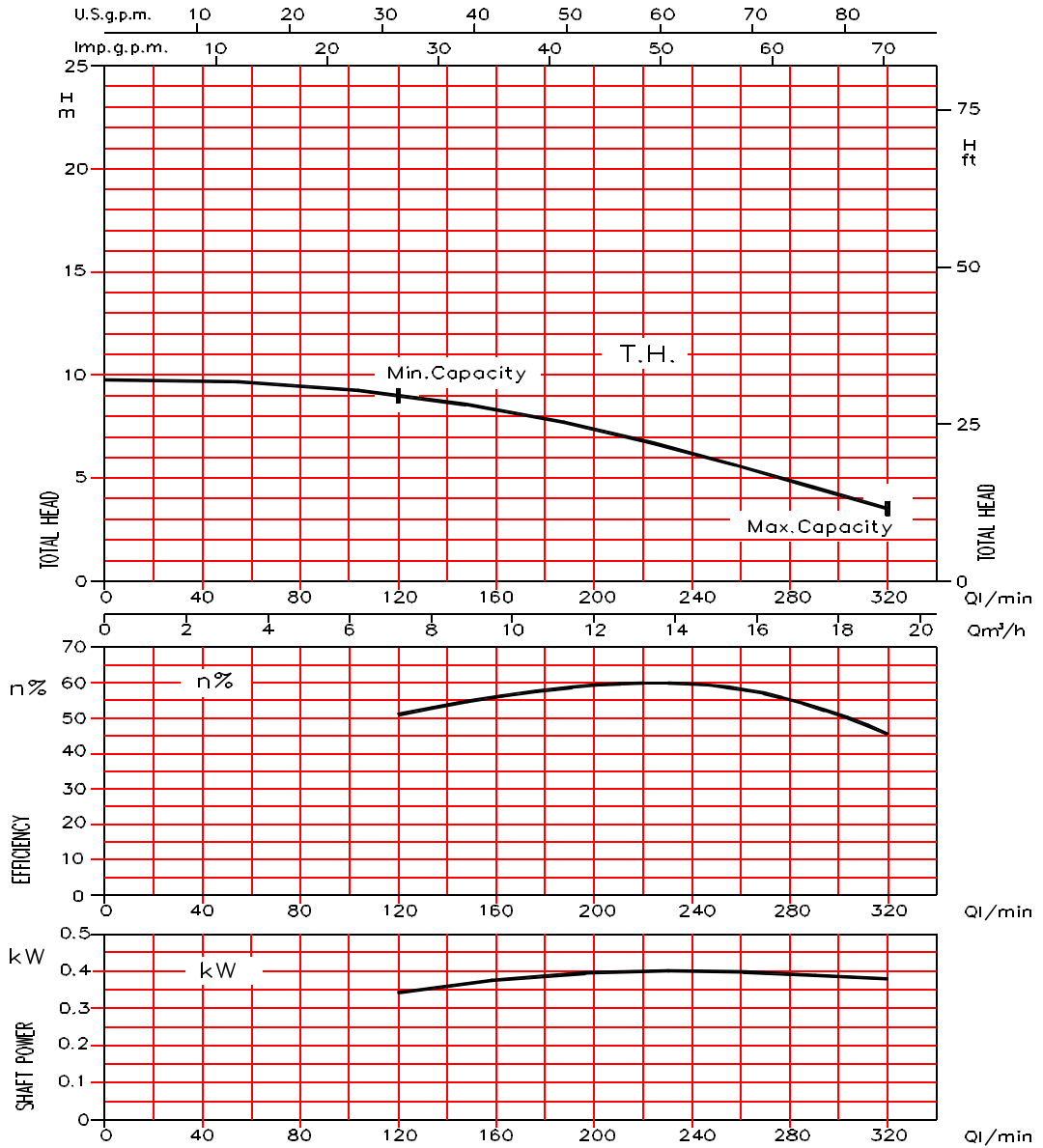
LPS 50/40 (0.4 kW) - LPS 50/40M (0.4 kW) - Impeller diameter = 95 mm
