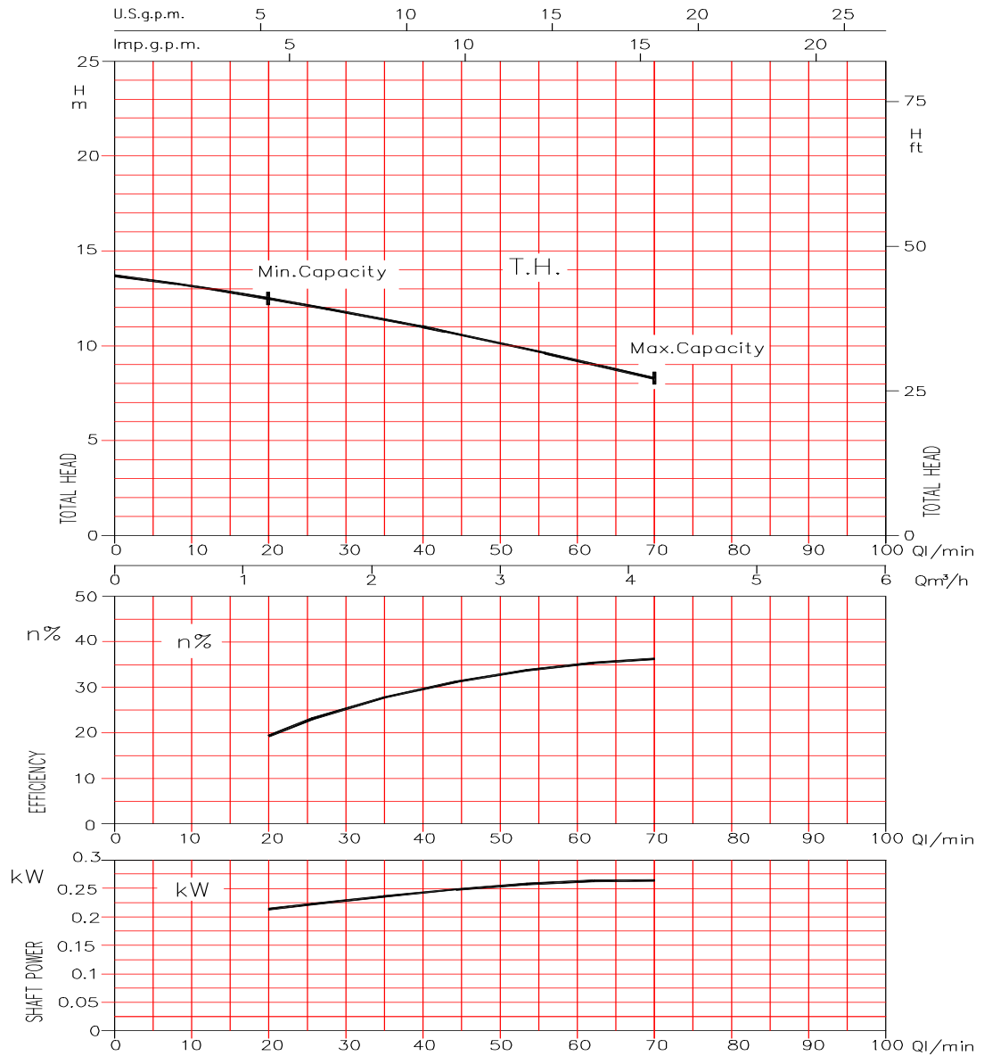
LPS 25/25 (0.25 kW) - LPS 25/25M (0.25 kW) - Impeller diameter = 114 mm
