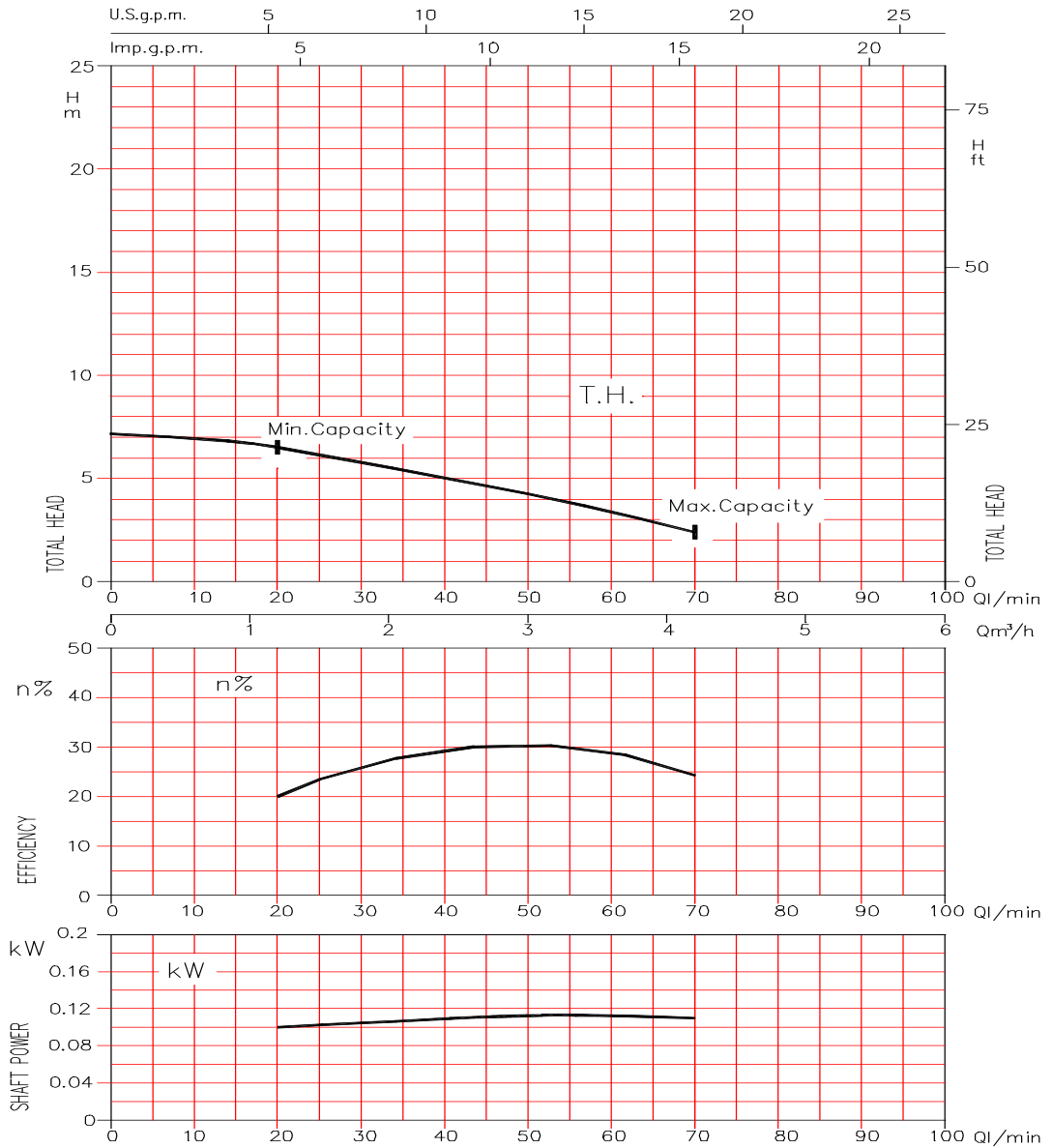
LPS 25/08 (0.08 kW) - LPS 25/08M (0.08 kW) - Impeller diameter = 84 mm
