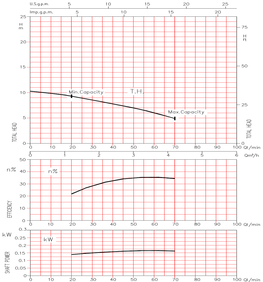
LPS 25/15 (0.15 kW) - LPS 25/15M (0.15 kW) - Impeller diameter = 98 mm
